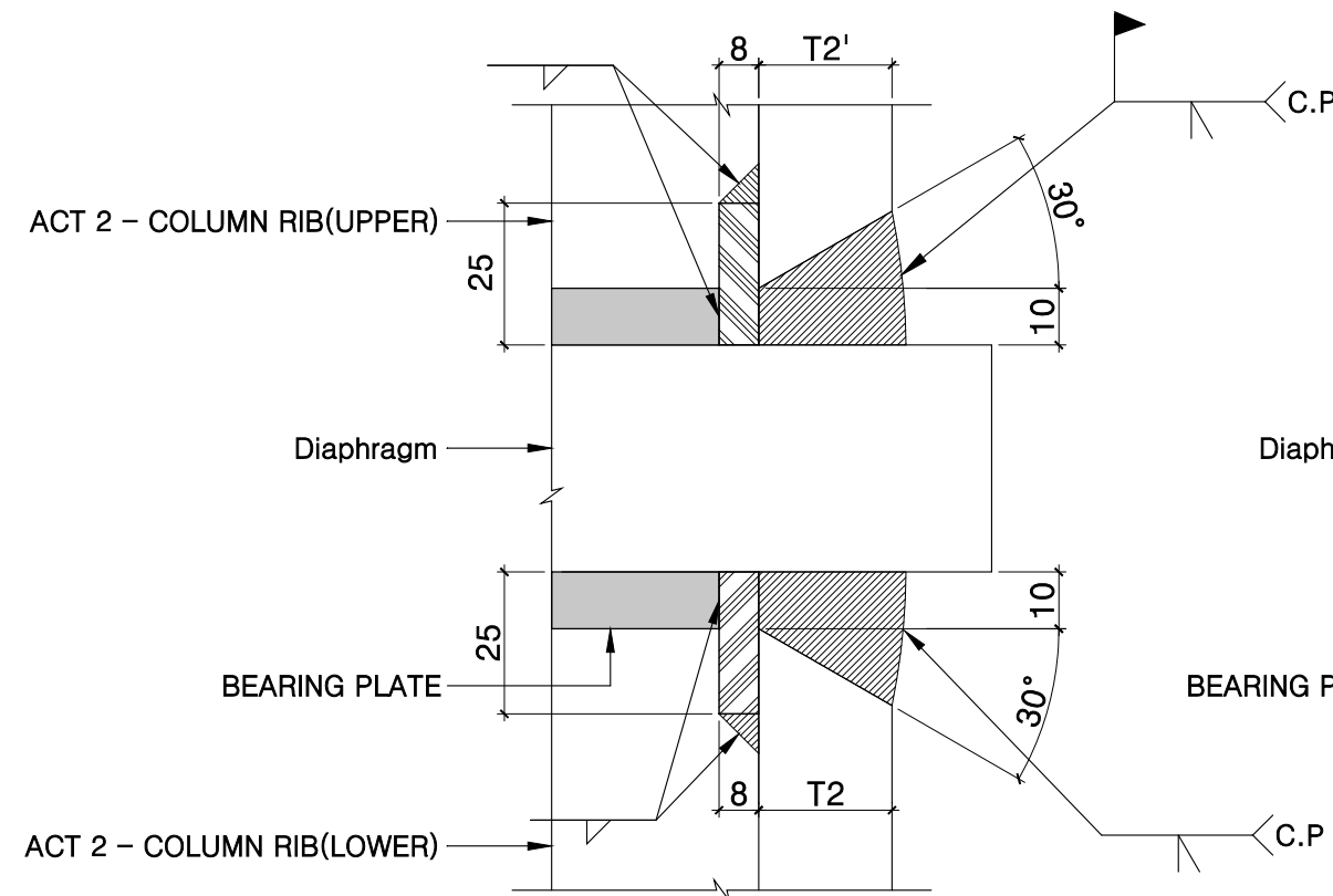
SECTION A-A'-1
