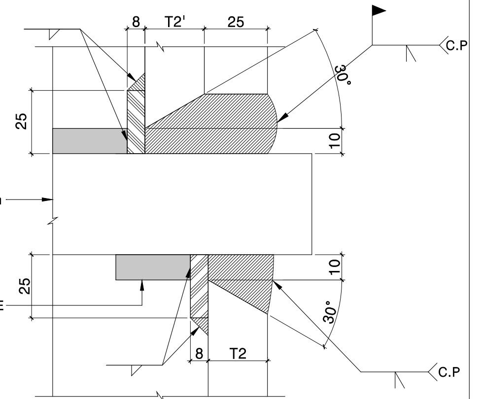
SECTION A-A'-2
