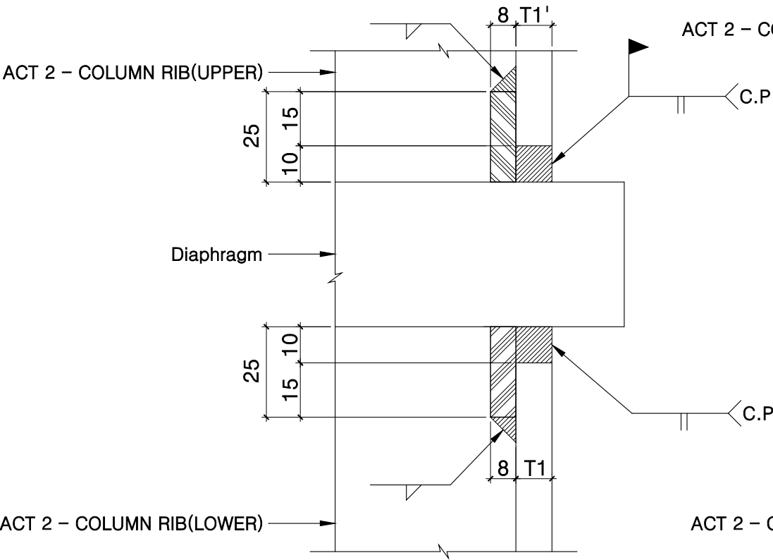
SECTION B-B'-1 (In Case of the Same Size of Upper & Lower COLUMN)
