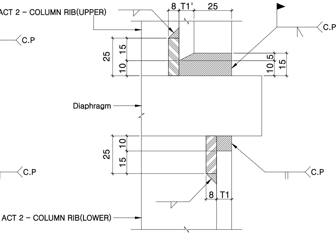
SECTION B-B'-2 (In Case of the Different Size of Upper & Lower COLUMN)
