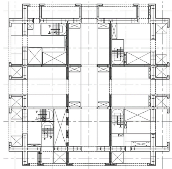
Figure 8. The core plan at lower floors.
