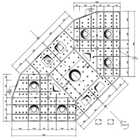
b) Cross section at zone 0 (60m2)
